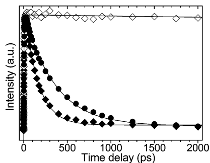
Figure 6. Temporal dependence of the transient absorption intensity for HPPP in MeCN ( \diamond ) and H 2 O/MeCN (1:1) ( \blacklozenge ) at \sim 400 nm. Data labeled by the filled circles are from the intensity of the HPDP TA spectra at \sim 400 nm obtained in the H 2 O/MeCN (1:1) solvent. Solid lines indicate kinetics fitting using a one exponential function to fit the experimental data points.
