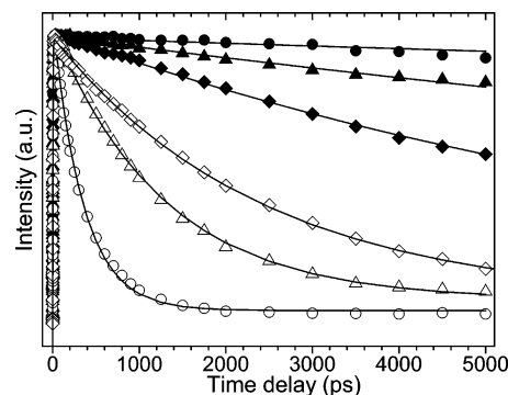
Figure 7. Triplet decay kinetics observed for HPDP by transient absorption measurements in water/MeCN mixed solvent with water concentration of 0% ( \bullet ), 10% ( \blacklozenge ), 15% ( \diamond ), 25% ( \triangle ), and 50% ( \circ ). Data labeled by the filled triangles are obtained in a DMSO/CF 3 CH 2 OH (1:1 by volume) mixed solvent. Solid lines indicate dynamic fittings using a one exponential decay function to the experimental data points.
