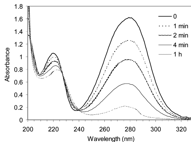
Figure 1. UV/vis absorption spectra for the conversion from HPDP to HPA upon photolysis of HPDP in a H 2 O/MeCN (1:1) mixed solvent. The time periods the sample solution is exposed to the excitation laser pulse are labeled for each of the spectral traces.
